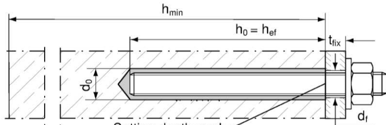
Anchor rod Pre-positioned anchor
