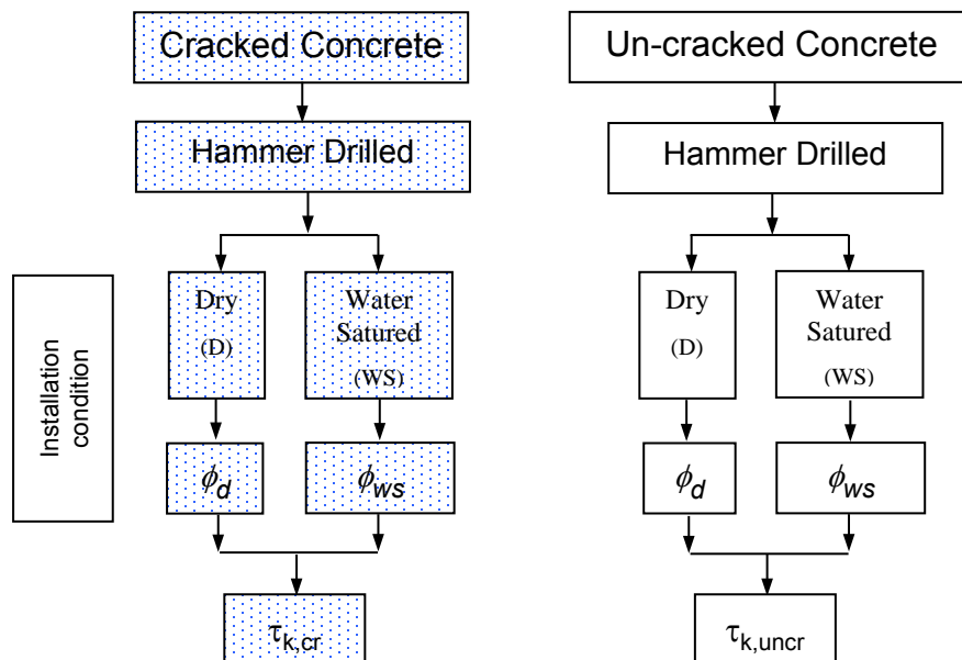
FIGURE 1—FLOWCHART STRENGTH REDUCTION FACTORS FOR DETERMINATION OF THE BOND STRENGTH
